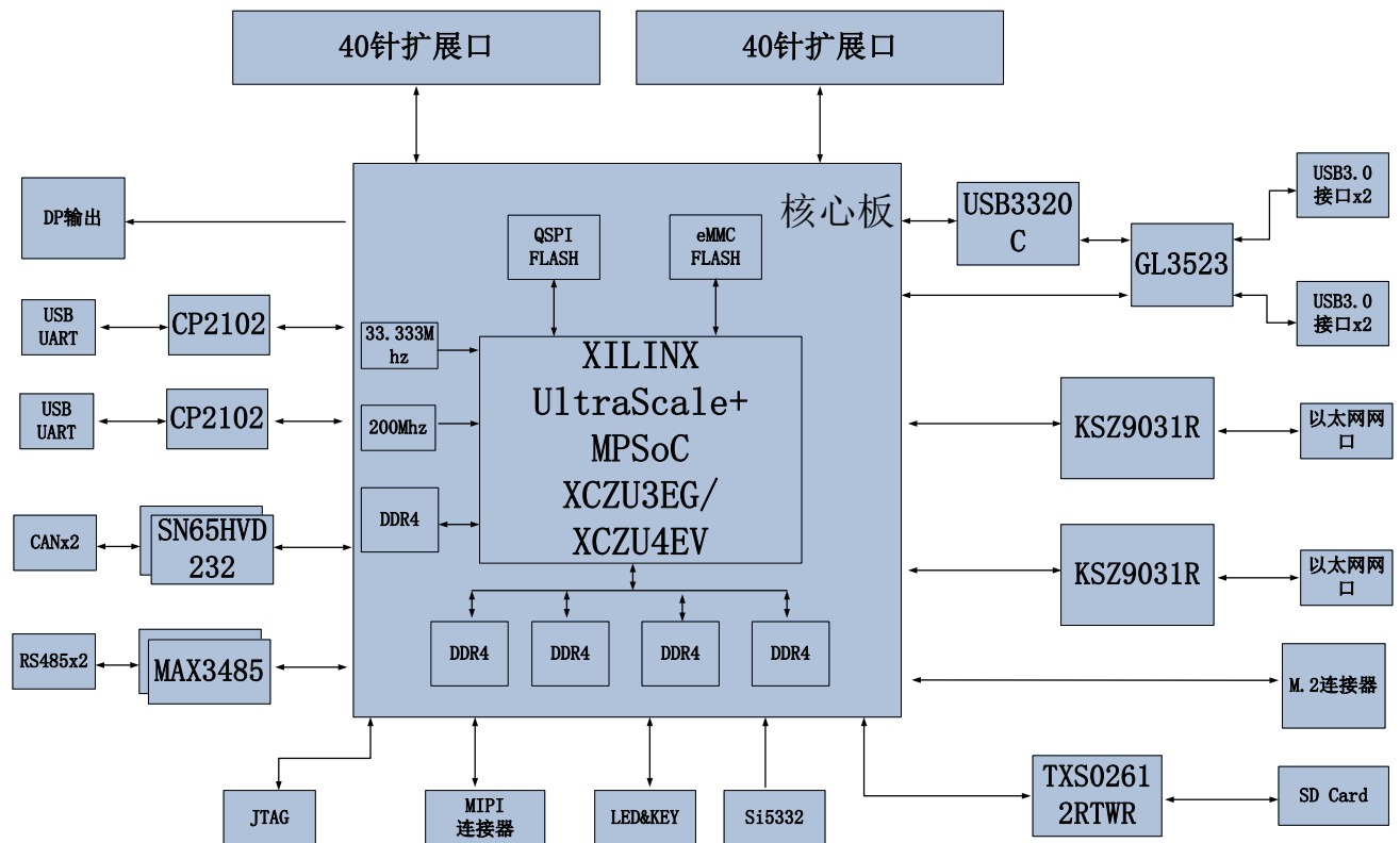
Figure 1-1-1: The Schematic Diagram of the AXU3EG
